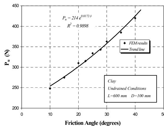
Fig.12- Soil friction angle effects on pull-out capacity of suction caissons in clay under undrained conditions.
