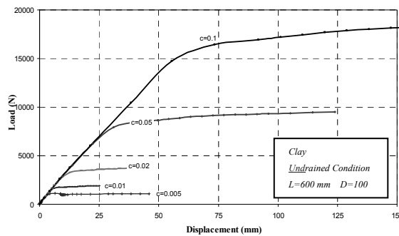
Fig.6- Soil cohesion effects on numerical pull-out responses of suction caissons in clay under undrained conditions
