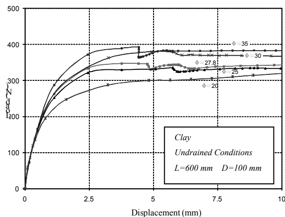
Fig.10- Soil friction angle effects on numerical pull-out responses of suction caissons in clay under undrained conditions.
