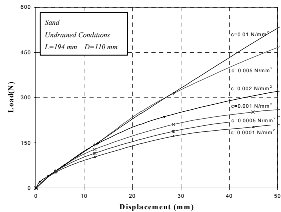
Fig.9- Soil cohesion effects on numerical pull-out responses of suction caissons in sand under undrained conditions.
