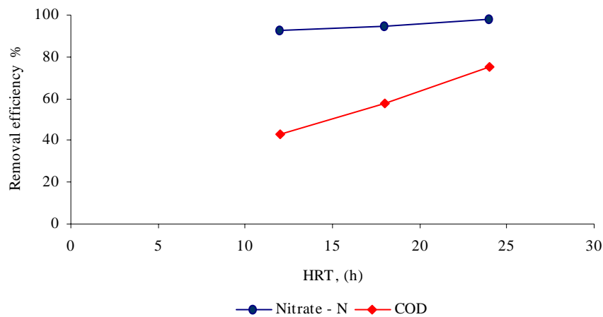
Fig. 6: Effect of HRT on removal efficiency (Carbon source: Ethanol, Influent NO 3 -N concentration: 50 mg/L)
