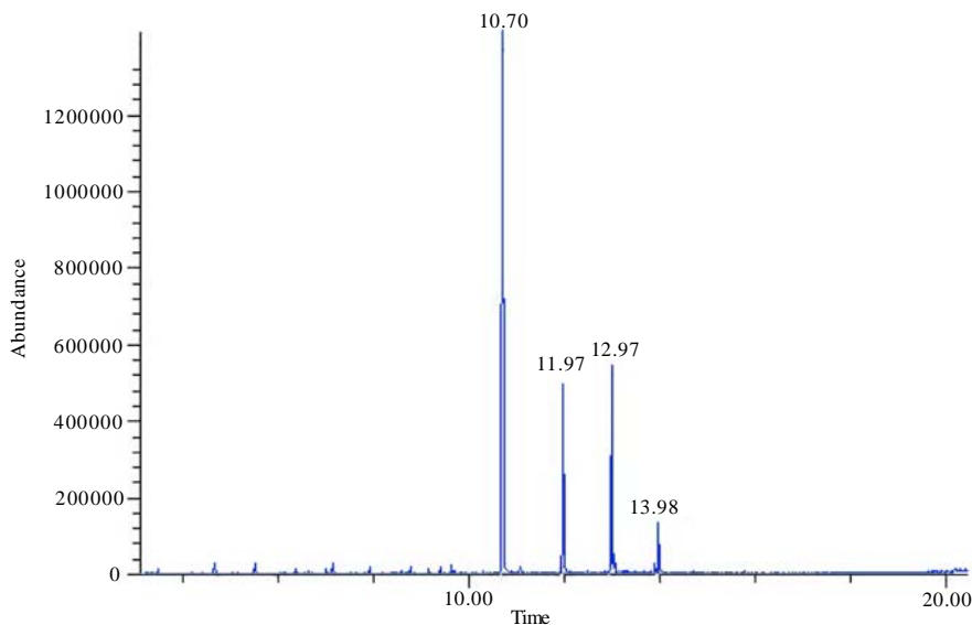
Fig. 3: GC chromatogram of Mokusaku-eki 2 (ME-II) sample; Column DB-5 with 0.25 mm ID, 0.25 µm film thickness used for analysis
