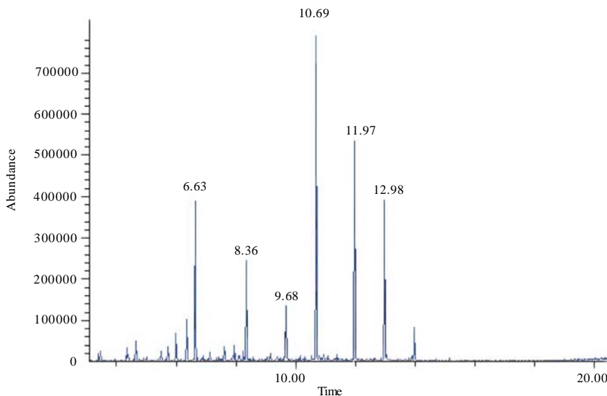
Fig. 2: GC chromatogram of Chikusaku-eki 2 (CE-II) sample; Column DB-5 with 0.25 mm ID, 0.25 µm film thickness used for analysis
