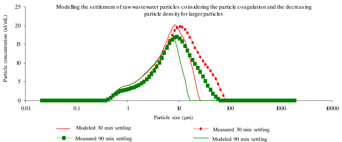
Fig. 10: PSD modeling results considering decreasing density for larger particles
