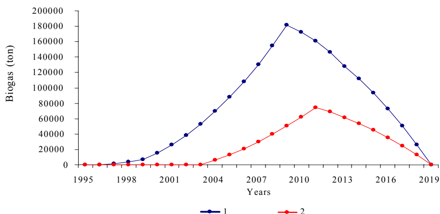
Fig. 1: Estimation of biogas emission at the municipal landfill sites: 1 – the landfill located in Tatarstan, 2 – the landfill located in Mytischki Region
