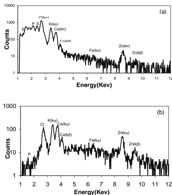
Figure 1. Typical spectrum for malignant type of human breast tissue, (a) for low Z elements (without absorber filter) and (b) for high Z elements with 175µ mylar absorber.
