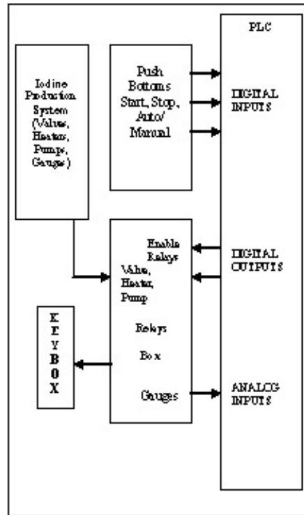
Figure 1. The automation system
