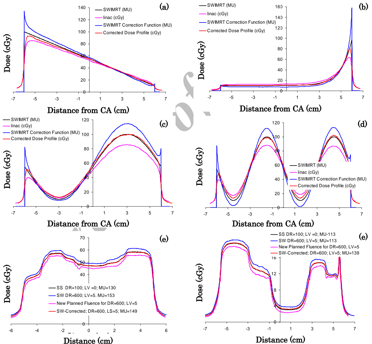
Figure 8. Illustrations of the agreement between the planned and corrected beams. A difference < 0.8% and < 0.5% was achieved for the geometrical and clinical beams, respectively. Geometrical profiles (a-d) are generated using the SWIMRT software. The clinical beams (e-f) were optimized by the step-and-shoot IMRT with Pinnacle 3 and converted using the SWIMRT to DMLC. Both beams were corrected using the SWIMRT and delivered using the Varian 21 EX linear accelerator with DR = 600 MU min -1 and LV = 5 cm s -1 .
