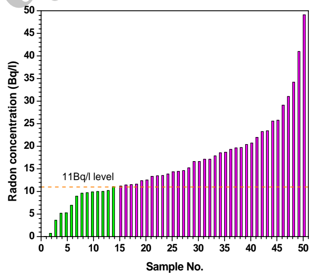
Figure 2. The radon concentration in various samples of Mashhad water (we sorted them increasingly).
