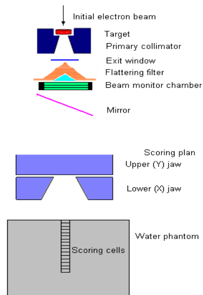
Figure 1. Schematic representation of the Monte Carlo models for the Varian 2100C/D linear accelerator geometry in photon mode.
