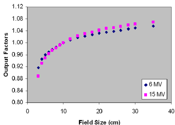
Figure 1. Variations of output factors with field size measured with farmer type ionization chamber and acrylic build up cap.
