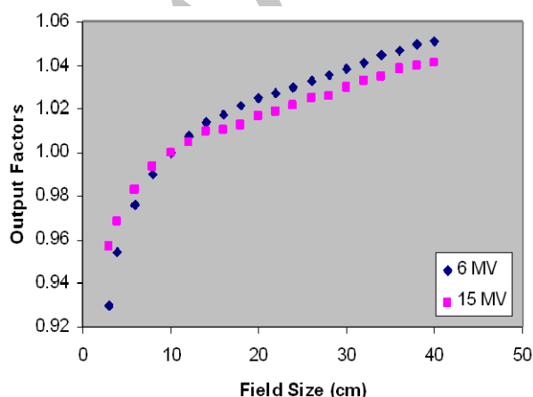
Figure 3. Variations of output factors with field size measured with compact cylindrical ionization chamber and brass build up cap.
