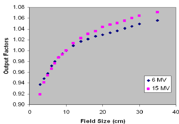
Figure 2. Variations of output factors with field size measured with compact cylindrical ionization chamber and acrylic build up cap.
