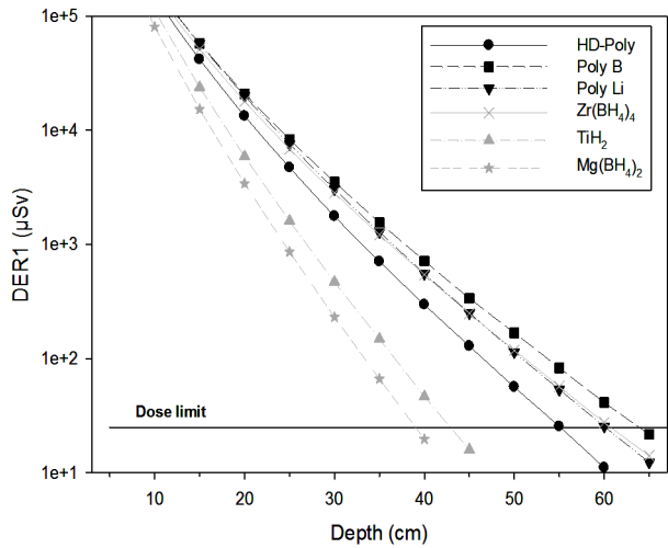
Figure 5. Comparison of DER1 for 6 neutron shielding materials for 241 Am/Be neutron source.
