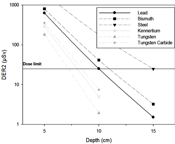
Figure 6. Comparison of DER2 for 6 gamma ray shielding materials for 241 Am/Be neutron source.
