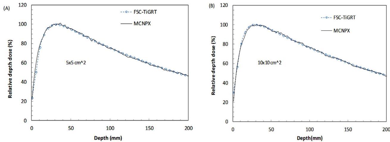
Figure 3. The comparison of relative depth doses from measurements and Monte Carlo Method in homogenous water phantom for two field sizes of (A) 5×5 and (B) 10×10 cm² for the 18 MV photon beam.
