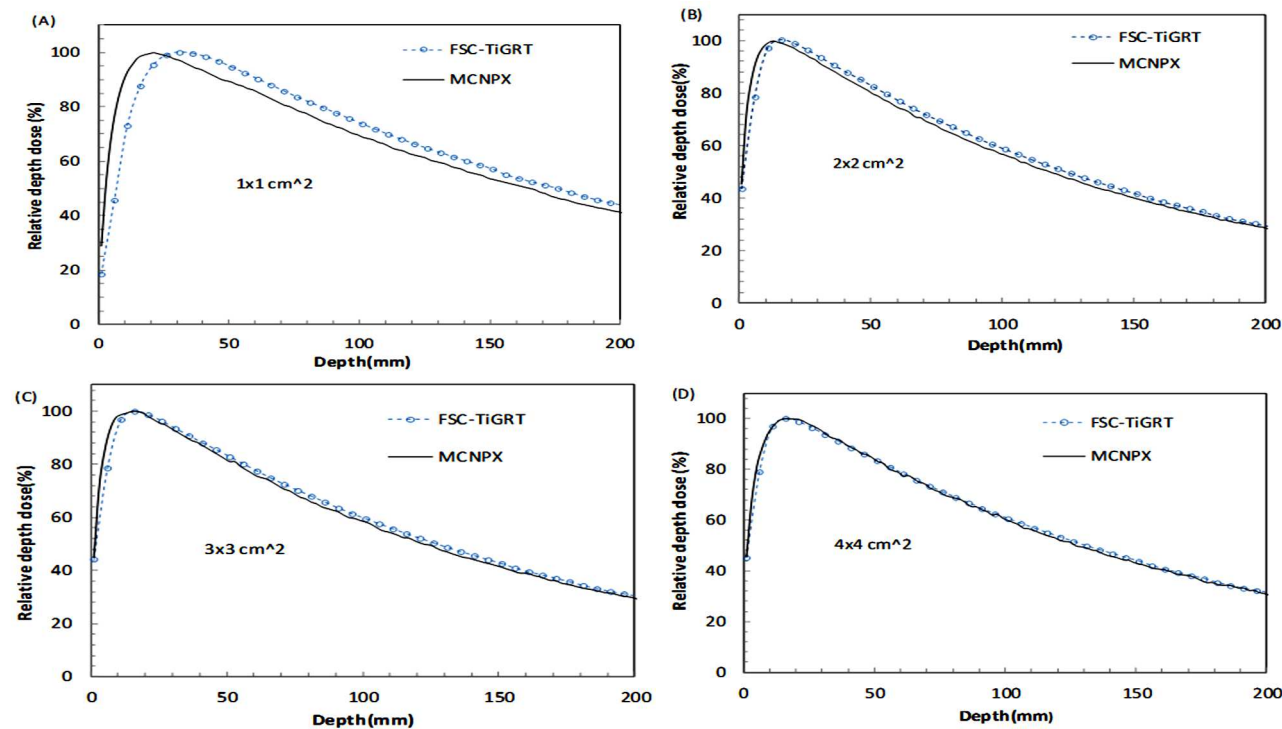
Figure 4. The comparison of relative depth doses calculated by full scatter convolution and Monte Carlo Methods in homogenous water phantom for different field sizes in the 6 MV photon beam. (A) 1×1 cm 2 (B) 2×2 cm 2 (C) 3×3 cm 2 (D) 4×4 cm 2 .
