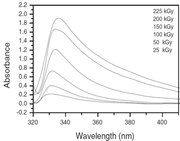
Figure 1. Absorption spectra of dimethyl sulfoxide diethyl fumarate for different irradiation doses (25-225 kGy) at concentration of 20% DEF and dose rate 30 kGy/h.
