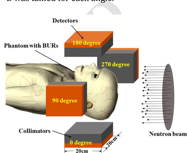
Figure 1. Diagram of BNCT-SPECT system in the Monte Carlo simulation (the labeled angles represent the position of the rotated detector).
