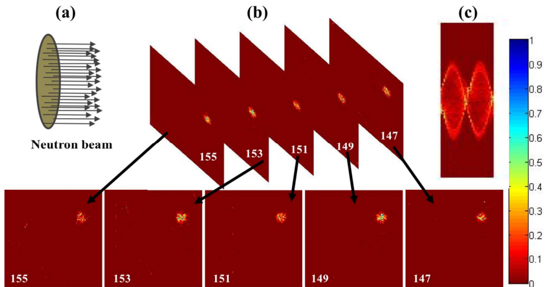
Figure 7. Reconstructed tomographic images of 1 cm diameter tumor by 4 iterations (the number in the figure indicates the layer number). (a) illustration of the neutron beam direction; (b) reconstructed image; (c) simulated sinogram.
