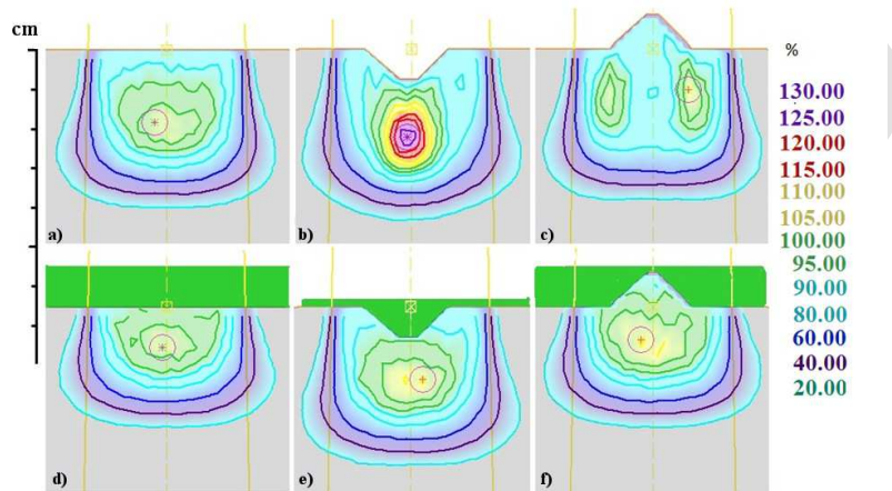
Figure 1. For an electron beam, the bolus reduces dose inhomogeneity. a) An example of a dose distribution for an electron beam of 9 MeV, which irradiates a field of 4×4 cm. b) A dose distribution for the same beam, modified by the gap in the phantom (the skin surface). Below the gap, the dose is significantly increased (in this geometry, by about 25%). c) A dose distribution for the same beam, modified by the convex surface in the phantom (the skin surface). Below the convex region, the dose is decreased (in this geometry, by about 20%). d) A dose distribution modified by a bolus between the tissue and the electron source. The range of electrons in the phantom (the tissue) is reduced by the thickness of the bolus. The build-up region is moved into the bolus, which increases the dose at the phantom surface (skin surface) to a value near 100%. e) A dose distribution modified by using a bolus that fills the surface gap. The region of high dose disappears. f) A dose distribution modified by using a bolus that compensates for the surface bulge. The region of reduced dose disappears. In addition, the range of electrons in the phantom (the tissue) is reduced.
