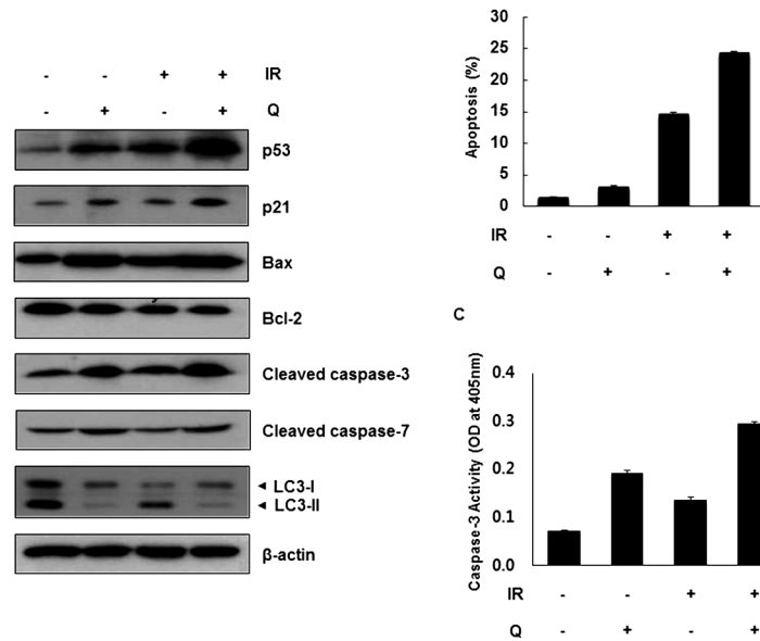
Figure 4. The effect of combined treatment of quercetin and IR on apoptosis in HepG2 cells. (A) HepG2 cells were exposed to quercetin (100 \mu M) for 48 h with or without irradiation (10 Gy), and the protein expressions of p53, p21, Bax, Bcl-2, cleaved caspase -3, cleaved caspase-7 and LC3 were determined by western blotting. Forty micrograms of cellular extract per lane was separated on 12% SDS-PAGE gel. Equal protein loading and protein transfer were confirmed with anti- \beta -actin antibody. (B) Cells were exposed to quercetin (100 \mu M) for 48 h with or without 10 Gy irradiation. The cells were then harvested and prepared for PI staining as described in “Materials and Methods”. Sub G1 population was analyzed using flow cytometry and Sub G1 population was counted as apoptotic cells. (C) The effect of the combined treatment of quercetin and IR on the caspase-3 activity. HepG2 cells were irradiated with 10 Gy and treated with 100 \mu M quercetin for 48 h. Data represents the average results of three independent experiments (mean \pm SEM).
