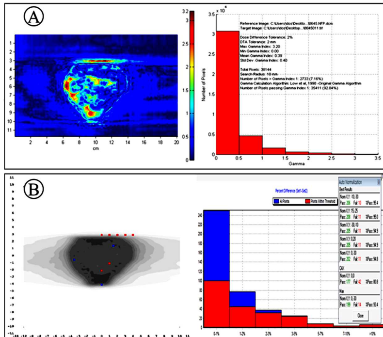
Figure 3. A histogram of the measured and calculated absolute dose differences for 25 patients.
