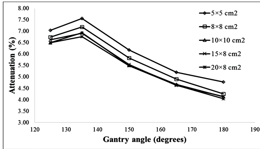
Figure 3. Measured 6 MV beam attenuation of the couchtop at different gantry angles and field sizes.
