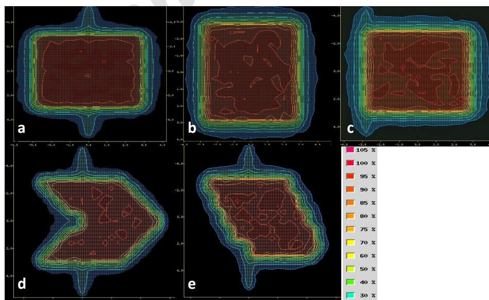
Figure 1. Beams of view of isodose curves measured for square field 5x5, Position of the contact of the closed leaves at (a) X=0. (b) X=-2.5. (c) X=-10. (d) and (e) irregular fields of 25 cm 2 , Position of the contact of the closed leaves at X=0.
