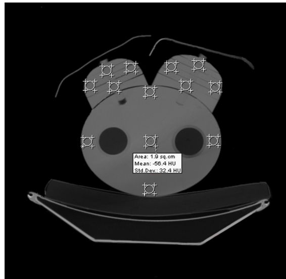
Figure 2. The CT gram presented for image analysis of Bismuth-Silicon shields on the chest phantom with selected ROIs. The average HU value and noise were determined for the marked places with an area of 1.9 cm 2 .
