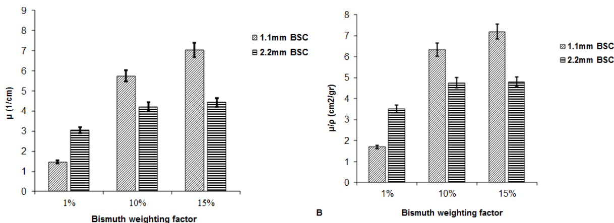
Figure 1. linear attenuation coefficient ( \mu , 1/cm). with ( \pm SD) as shown in A. Mass attenuation coefficient ( \mu/\rho , cm 2 /gr), as shown in B for in BSC (Bismuth Silicone Composite) shields in 1.1 and 2.2 mm thicknesses on the chest phantom during Chest CT.
