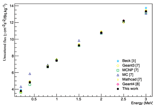
Figure 8. The unscattered flux ( \text{cm}^{-2}\text{s}^{-1}/\text{Bqkg}^{-1} ) obtained using ANN-MC method compared to previous works. Statistical discrepancy does not exceed 1%.
