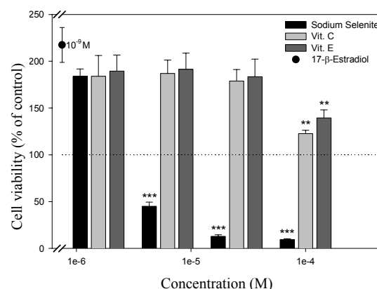
Figure 3. Effects of antioxidants on proliferation induced by 17- \alpha -estradiol on T47D cells.
