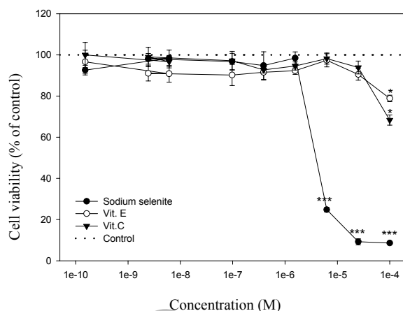
Figure 2. Effects of antioxidants on growth of T47D cells.
