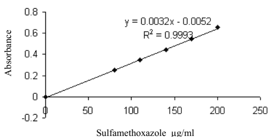
Figure 1. Calibration curve for SMX at 271 nm.
