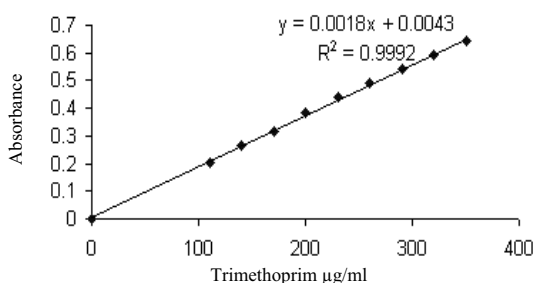
Figure 2. Calibration curve for TMP at 271 nm.
