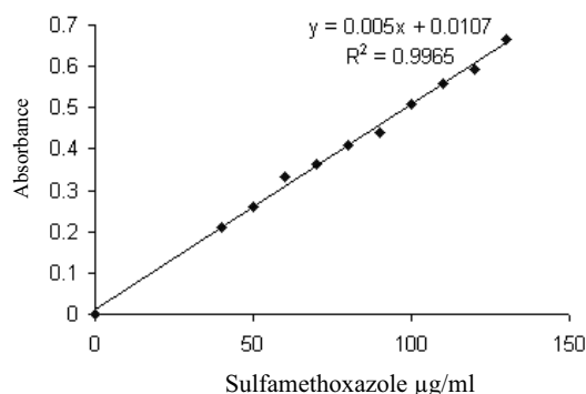
Figure 3. Calibration curve for SMX after diazotization and coupling with 2-naphthol at 482 nm.
