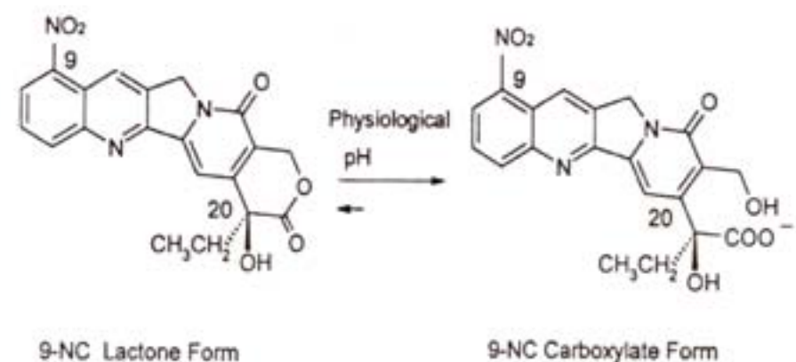
Figure 1. Chemical structures and equilibrium reaction between the lactone and carboxylate forms of 9-nitrocamptothecin (9-NC).
