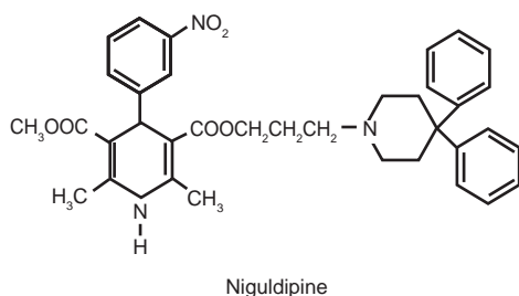
Figure 1. Niguldipine.
