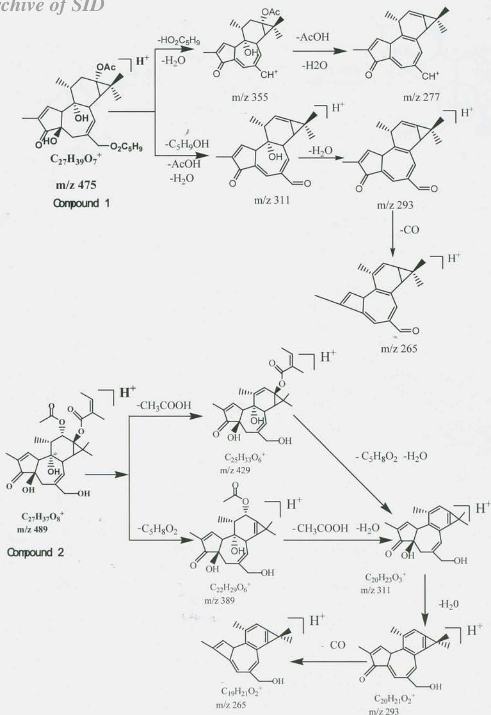
Figure 3. Proposed fragmentation pathways and characteristic ions of compound 1 and compound 2.
