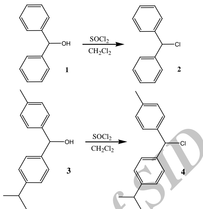
Figure 3. Synthesis of intermediates 2 and 4.
