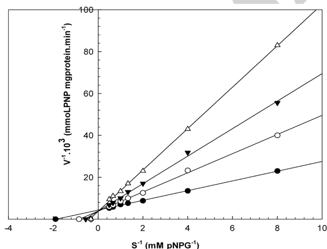
Figure 3. Lineweaver-Burk plots derived from the inhibition of \alpha -glucosidase by 1,8-cineole. \alpha -glucosidase was treated with each stated concentration of pNPG (0.125-2 mM) in the absence and presence of 1,8-cineole. The concentrations of 1,8-cineole were: (●) no inhibitor; (○) 0.130 \mu\text{L/mL} ; (▼) 0.520 \mu\text{L/mL} ; and (Δ) 1.260 \mu\text{L/mL} . The enzyme reaction was performed by incubating the mixture at 37°C for 30 min.
