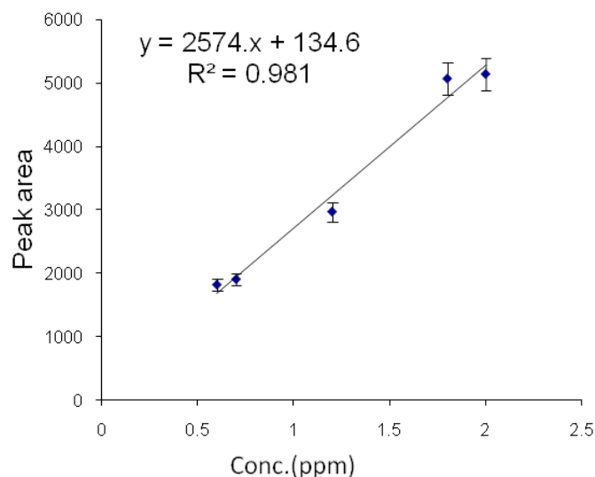
Figure 8. Diazinon calibration curve.
