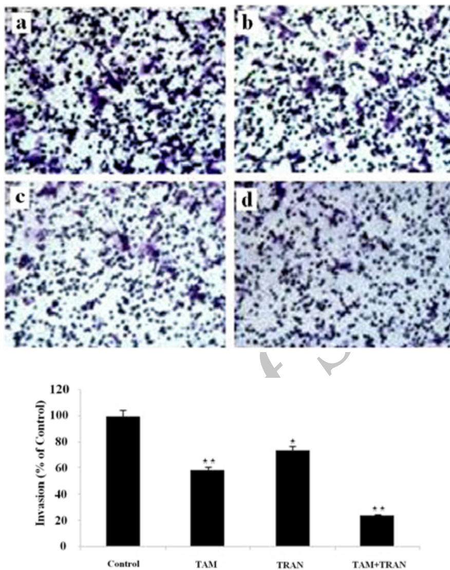
Figure 5. Inhibition of invasion in Matrigel invasion assay induced by TAM and TRAN or in combination alone on MCF-7 cells. (A) Phase micrograph of invading MCF-7 cells. a The control group; b MCF-7 cells treated with 2 \mu M TAM; c MCF-7 cells treated with 200 \mu M TRAN; d MCF-7 cells treated with combination (B)Quantification of cell invasion shown in (A). The data of t-test are shown as mean \pm S.E.M (*p < 0.05; **p < 0.01; ***p < 0.001).
