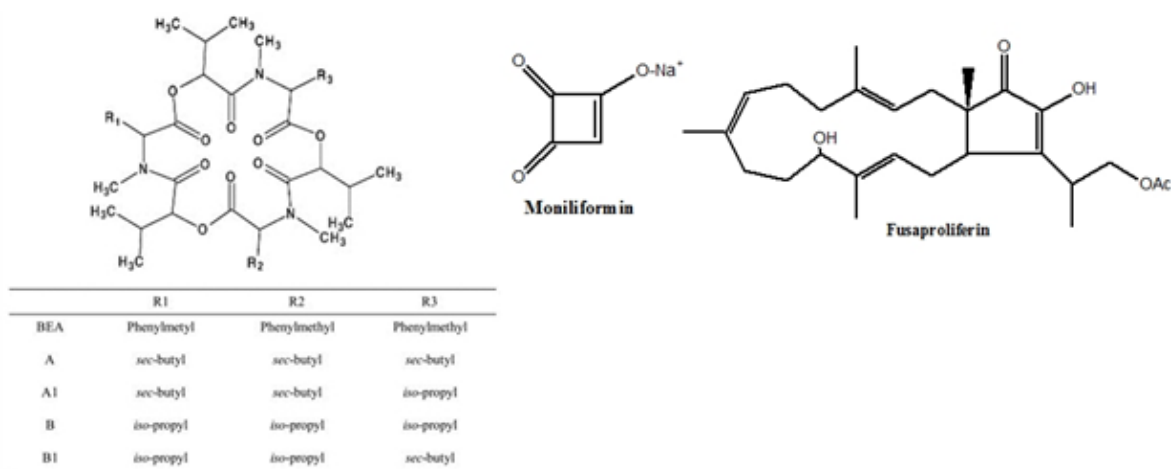
Figure 1. The chemical structures of beauvericin (BEA), enniatins (A, A1, B and B1), moniliformin and fusaproliferin.
