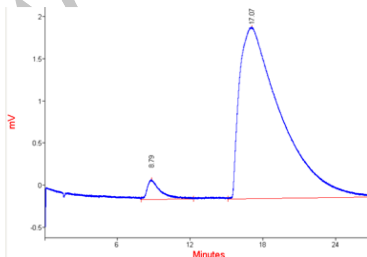
Figure 6. HPLC chromatogram of released berberine solutions (300 µg/ml).
