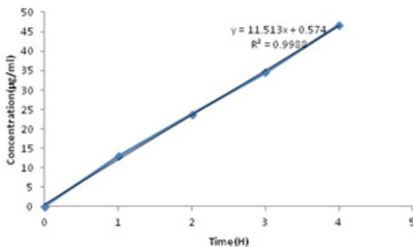
Figure 3. Diagram of released berberine concentrations in the first 4 hours ( \text{SD} = \pm 1\% ).
