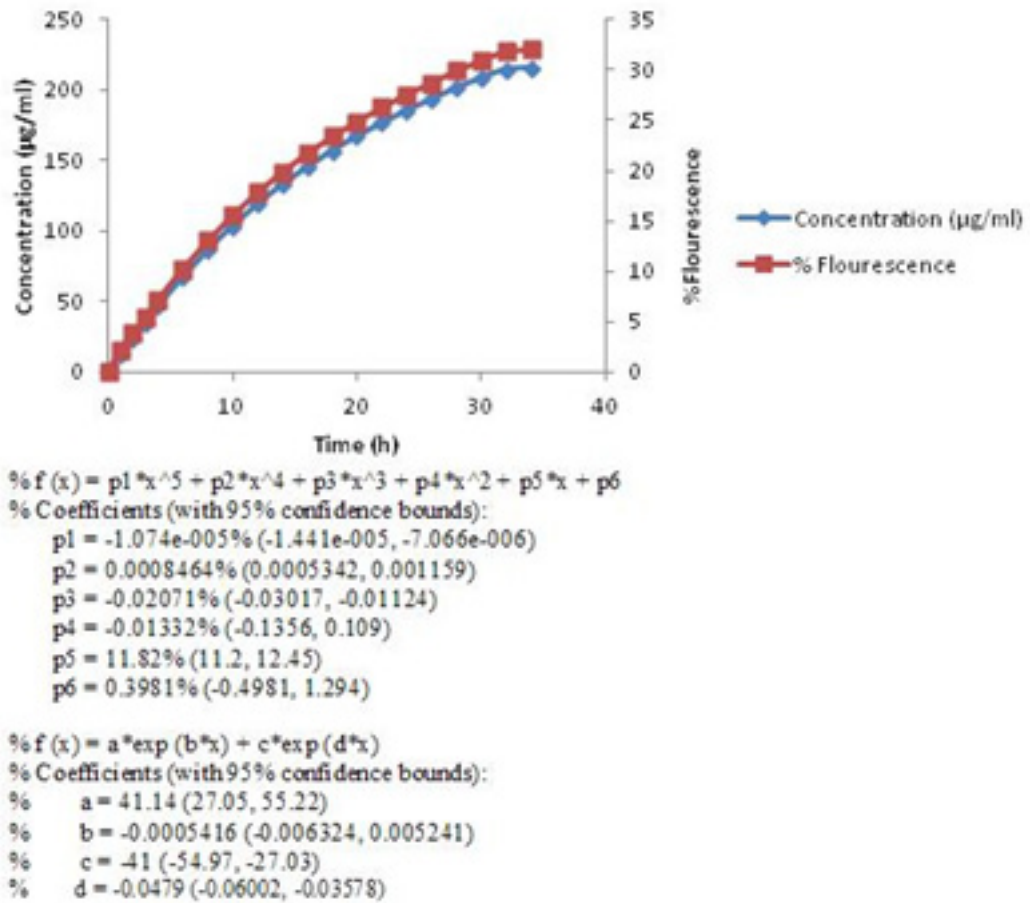
Figure 2. Release profile of encapsulated berberine (First equation under the curve is based on berberine % Fluorescence and the second one is based on berberine concentration ( \mu\text{g/ml} )).
