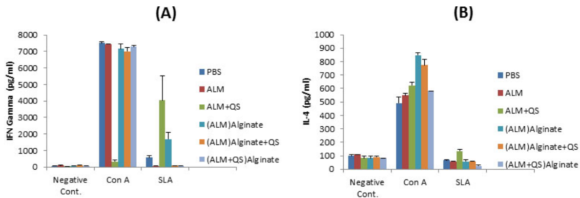
Figure 2. Splenic T-cell responses of BALB/c mice immunized SC, three times in 3 weeks intervals, with (ALM+QS)_{ALG} (ALM) ALG +QS, (ALM)_{ALG} , ALM+QS, ALM or PBS. Twenty days after the last booster, their spleens were removed and the splenocytes were stimulated in vitro with either SLA (5 mg/ml) or SLA (10 mg/ml), concanavalin A (2.5 mg/ml), or with no stimulation. Production of IFN- \gamma (A) and IL-4 (B) were assessed on culture supernatants collected at 72 h of in vitro incubation using sandwich ELISA method. Cells from 3 mice per group were pooled. Each bar represents the mean and SEM of triplicate wells.
