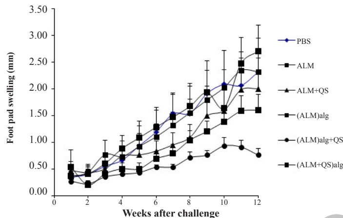
Figure 1. Footpad swelling in BALB/c mice immunized SC, three times in 3 weeks intervals, with (\text{ALM}+\text{QS})_{\text{ALG}} , (\text{ALM})_{\text{ALG}}+\text{QS} , (\text{ALM})_{\text{ALG}} , ALM+QS, ALM or PBS, after challenge with virulent L. major promastigotes. The mice were challenged in the left footpad with 1.5 \times 10^6 L. major promastigotes, 3 weeks after the last booster. The footpad thickness of mice was then measured on both footpads for 14 weeks. Each point represents the average increase in footpad thickness \pm S.E.M. ( n = 7 ).
