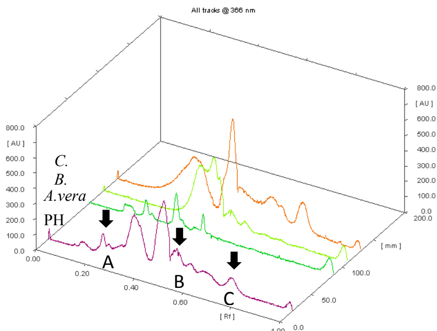
Figure 4: HPTLC fingerprint of Poly Herbal Paste including Aloe vera ; Boswellia carteri ; Commiphora myrrha ; and the plant extracts. Arrows show the characteristic peaks of the plant extracts in PHP chromatogram (A: Aloe vera ; B: Boswellia carteri ; C: Commiphora myrrha )
