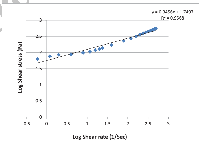
Figure3. The linear plot of log shear stress-log shear rate for Poly Herbal Paste, (containing aloe, myrrh and frankincense), (n = 3, data points are presented as mean \pm SD).
