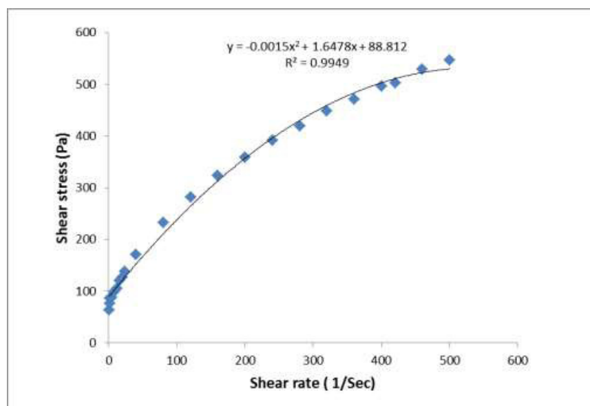
Figure1. Rheogram of Poly Herbal Paste, (containing aloe, myrrh and frankincense), showing the presence of a plastic behavior. (n = 3, data points are presented as mean \pm SD).
