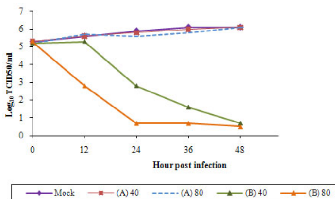
Figure 2. Inhibition of H9N2 influenza virus replication in the presence of different concentrations of Sambucus nigra (EF) extract was determined. The titer of virus in A549 supernatants was assayed by TCID 50 in trials (A) and (B) with 40 and 80 µg/mL of EF compared to the virus-infected and EF-untreated cells (mock).
