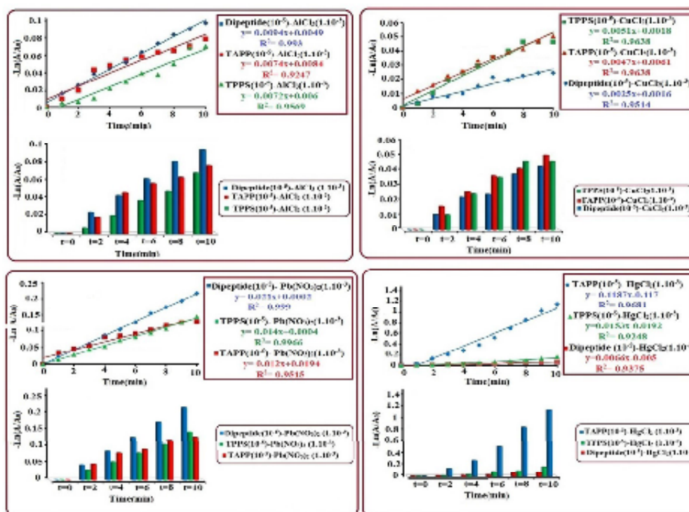
Figure 1. Kinetics study of chelating reactions of dipeptide (histidine-β-Alanine), TAPP and TPPS 4 ( 10^{-5} M) with AlCl 3 , CuCl 2 , Pb(NO 3 ) 2 and HgCl 2 ( 10^{-3} M).
