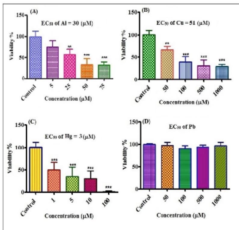
Figure 2. Cytotoxicity of different concentrations of Al 3+ , Cu 2+ , Hg 2+ and Pb 2+ on human lymphocytes. Viability of lymphocytes after treatment with Al 3+ (A), Cu 2+ (B), Hg 2+ (C), Pb 2+ (D) for 12 h. **P<0.01 and ***P<0.001
