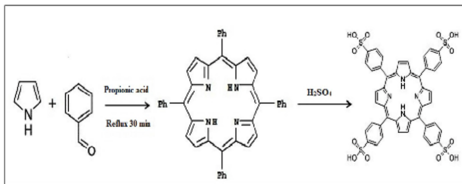
Scheme 3. Steps of Tetrakis(4-sulfonatophenyl)porphyrin (TPPS 4 ) synthesis.
