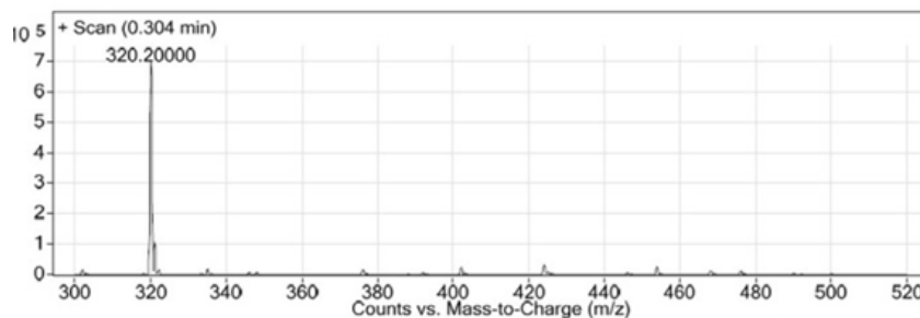
Figure 6. LC-MS chromatogram of synthesized Glu-Urea-Lys (EUK).
