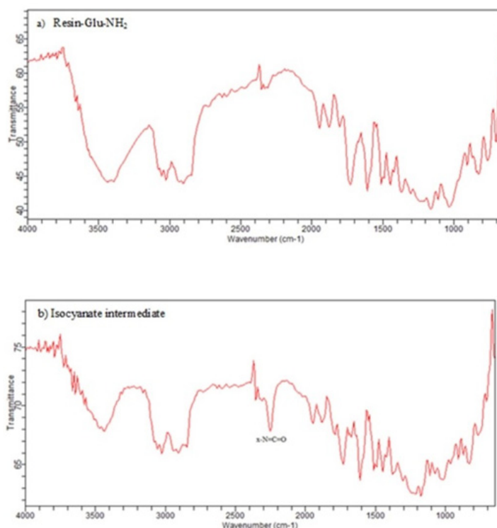
Figure 8. IR spectra of a) Deprotected glutamate bound to wang resin b) The corresponding isocyanate intermediate on wang resin. X-N=C=O stretch is seen in the 2270\text{ cm}^{-1} region of the IR (b) while it is absent in IR spectrum of resin-Glu-NH 2 (a).
