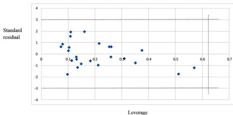
Figure 2. The William plot for the SW-MLR model.
