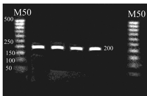
Figure 1. Amplification of a 200 bp fragment from exon 4 of the gGH gene in Talli goat. Molecular marker is represented by M50 (IsoGene, Russia) (500, 450, 400, 350, 300, 250, 200, 150, 100, and 50bp).
