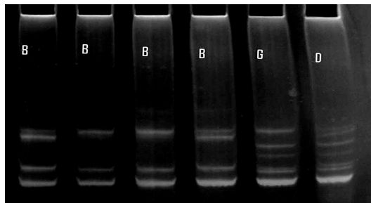
Figure 2. Some genotypic patterns at exon 4 of the gGH . B, D and G are SSCP patterns for studied goats.
