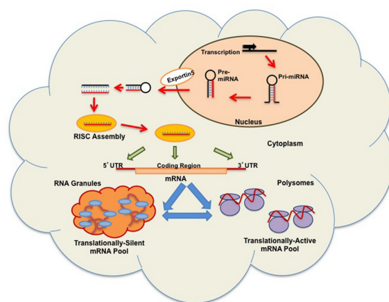
Figure 1. Translational Control via MicroRNAs and RNA Granules
