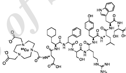
Fig 11. Chemical structure of ^{64}\text{Cu} -NOTA-AE105.
