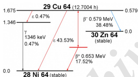
Fig 1. Detailed decay scheme for copper-64 radionuclide [2].
