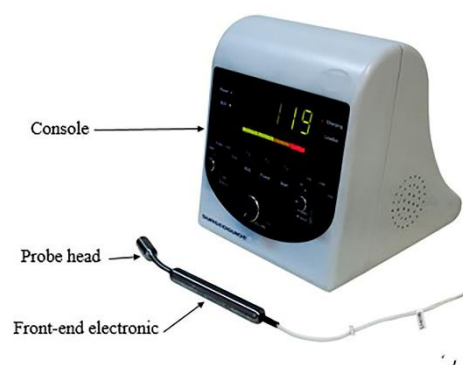
Fig 1. The gamma probe (SURGEOGUIDE II).
