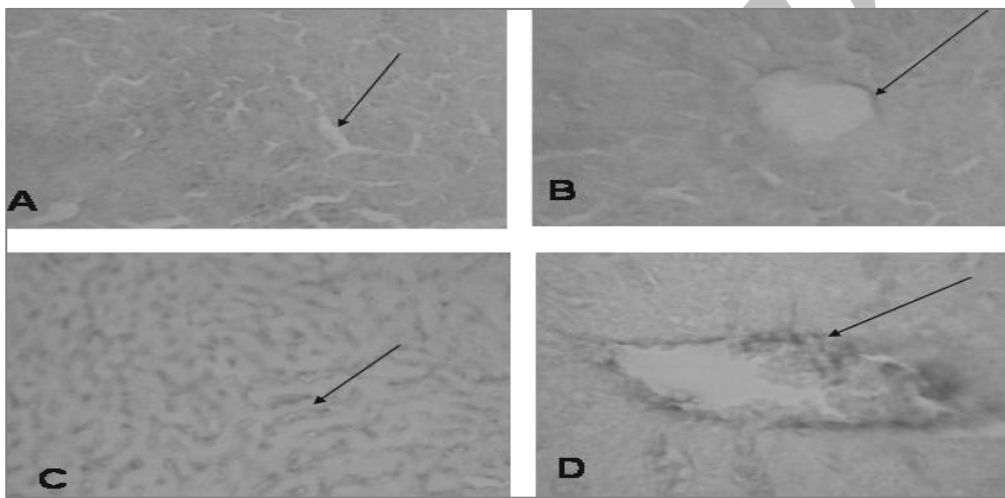
Figure 2. Immunohistochemistry findings in mouse liver after exposure to EMF. Controls show low staining in sinusoids (A) and pericentral vein region (B). Lcn2 was expressed in liver sinusoids (C) and around the central vein (pericentral) (D).
