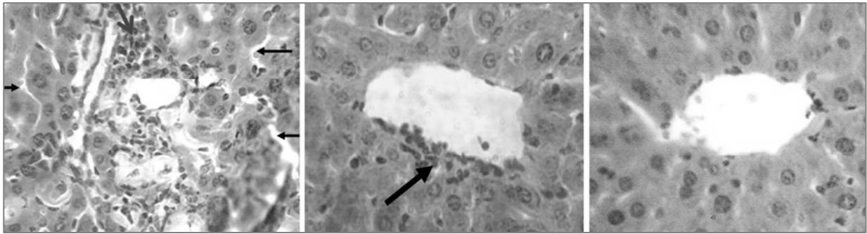
Figure 1. Histological findings in mouse liver tissue after exposure to EMF. Lymphocytes infiltration in portal space in the group exposed to EMF has been shown with brown arrow and black arrows point to sinusoidal dilation (a), \times 400 . Figure 1 (B) shows the pericentral venule lymphocytes infiltration in experimental group, \times 400 . Figure (C); Unexposed group (Control), \times 400 .
