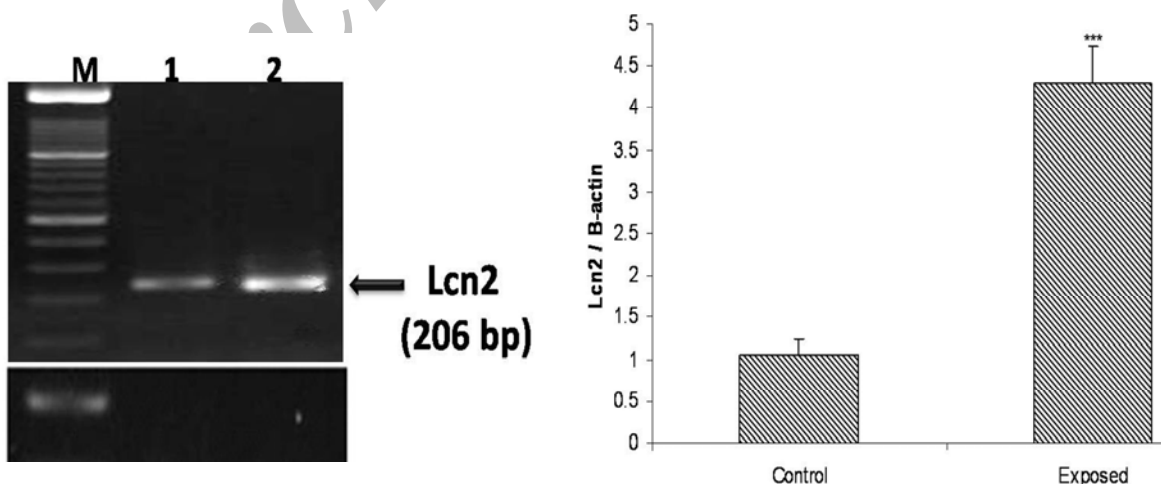
Figure 3. Expression of Lcn2 in mouse liver after exposure to EMF. Two months after exposure to 3mT and 50 Hz of EMF expression of Lcn2 was determined by semiquantitative RT-PCR. (a); After irradiation expression of Lcn2 was upregulated (lane 2) compared to the control, without exposure, (Lane 1). M, 100-bp marker. Lower figure indicates the expression of \beta - actin in both mice i.e. irradiated and control. M, 100-bp marker (b); Densitometric quantitation of the bands was performed by using UVIDoc software version 12.5. (Mean \pm SD; *** P < 0.001 ; number of replicates, 3).
