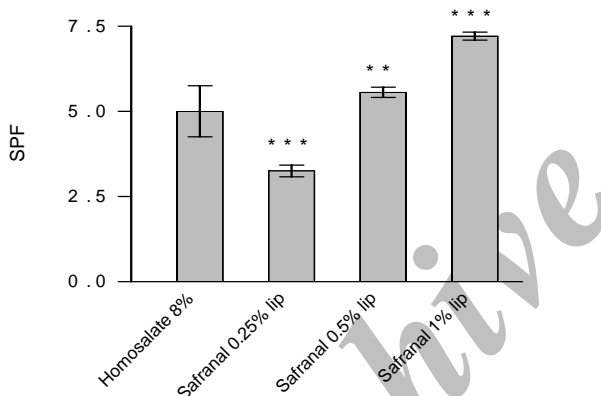
Figure 1. The SPF values of Lip-Safranal (0.25, 0.5 and 1%) and homosalate reference determined by diluted solution transmittance method. Values are mean±SD, n= 3; ** P < 0.01 , *** P < 0.001 .
