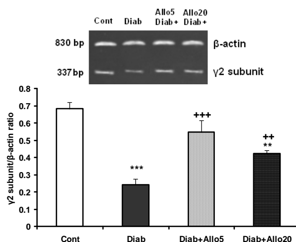
Figure 3. The level of \gamma 2 mRNA in dorsal portion of lumbar spinal cord in control, diabetic (Diab) and allopregnanolone-treated diabetic rats (Diab+ALLO). Each value in the graph represents the mean \pm SEM band density ratio for each group (n=5). \beta -actin was used as an internal control. ** P <0.01, *** P <0.001 versus control animals. ++ P <0.01, +++ P <0.001 versus diabetic group
