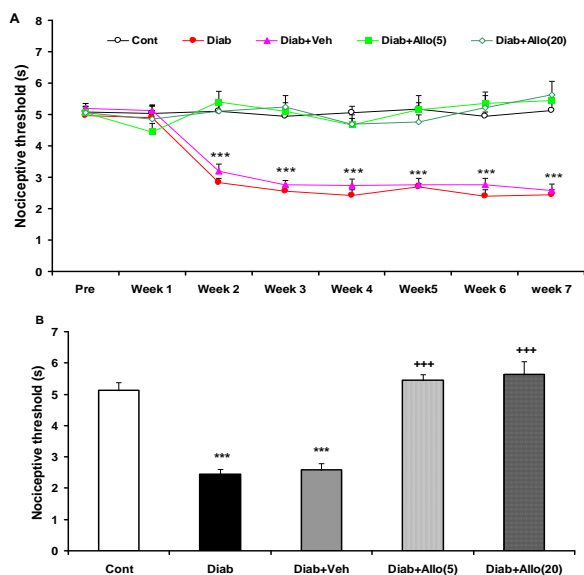
Figure 1. Effect of allopregnanolone (ALLO, 5 and 20 mg/kg) on the development of diabetes-induced thermal hyperalgesia during the time course of the study (A) and comparison of nociceptive threshold at the end (week 7) of the study (B) in rats. Values are expressed as the mean \pm SEM (n=6-8), *** P <0.001 versus control (Cont) group. +++ P <0.001 versus the diabetic group
