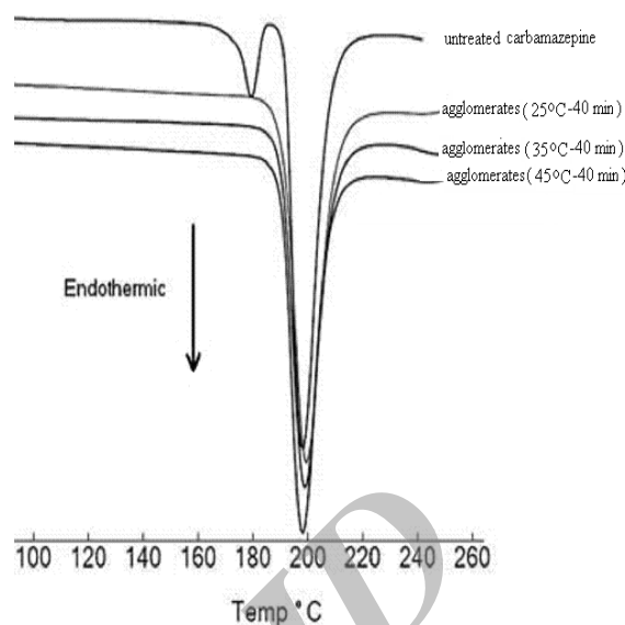
Figure 3. Differential scanning calorimetry thermograms of the agglomerates prepared at different temperatures
