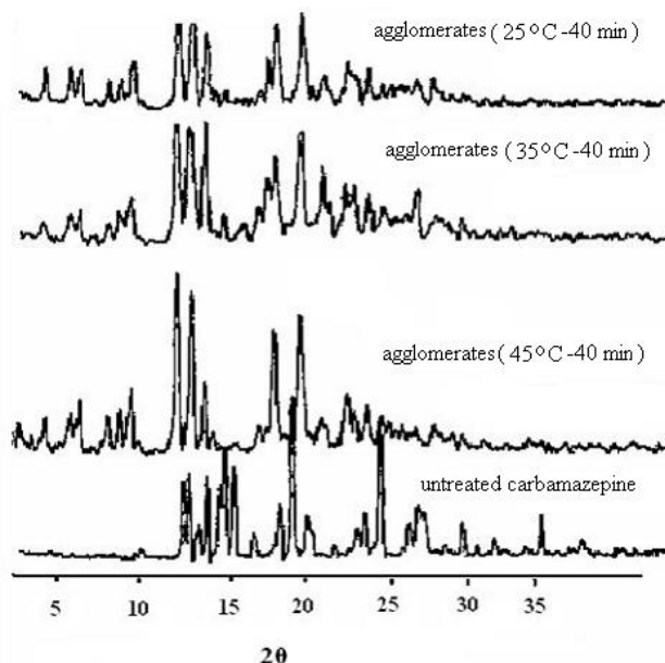
Figure 2. X-ray diffraction of agglomerates prepared at different temperatures
