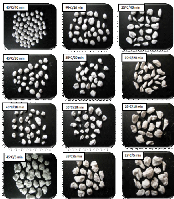
Figure 1. Photographs of the agglomerates prepared at different temperatures ( \times 8 )
