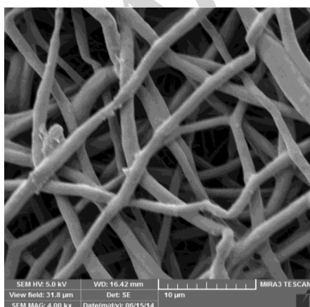
Figure 2. Architecture of electrospun PCL nanofiber scaffold as seen with a scanning electron microscope at 4.00KX
