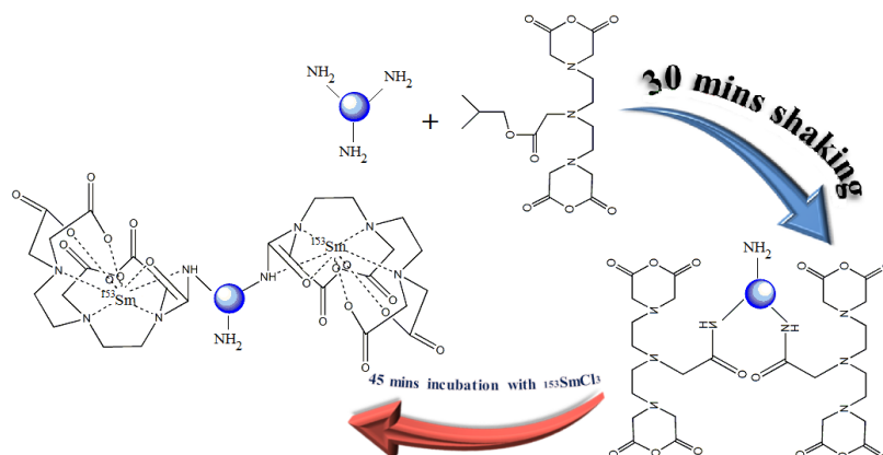
Figure 1. Schematic scheme of labeling procedure of Dextran coated iron oxide NPs with amine group conjugated with ccDTPA and labeled with ^{153}\text{Sm} finally
