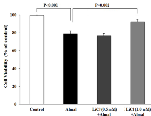
Figure 3. The effect of aluminum maltolate (Almal) on PC12 cell viability in the presence or absence of lithium chloride (LiCl). PC12 cells were treated with Almal (1 mM) in the presence or absence of LiCl (0.5 and 1.0 mM) and cell viability was evaluated using MTT assay. The represented data are mean±SD of at least three independent experiments and were analysed using one-way ANOVA followed by Tukey's post hoc test
