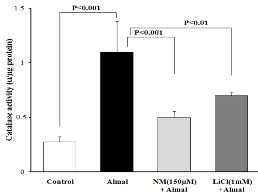
Figure 5. The effect of nimodipine (NM) and lithium chloride (LiCl) on catalase activity. PC12 cells were treated with aluminum maltolate (Almal) (1.0 mM), Almal+NM (1.0 mM+150 μM, respectively) and Almal+LiCl (1.0 mM and 1.0 mM, respectively). The represented data are mean±SD of at least three independent experiments and were analyzed using one-way ANOVA followed by Tukey's post hoc test
