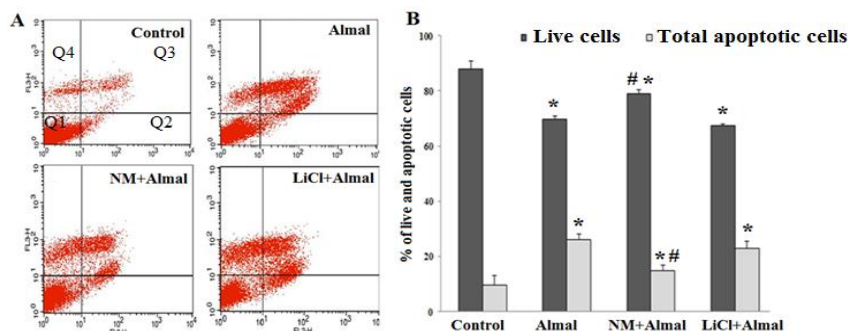
Figure 4. The effect of nimodipine (NM) and lithium chloride (LiCl) on aluminum maltolate (Almal)-induced apoptosis of PC12 cells. The flow cytometric graphs (A) and a histogram (B) illustrate percentage of live and apoptotic PC12 cells in various conditions. PC12 cells were treated with Almal (1 mM), NM(150 µm) +Almal (1 mM), and LiCl (1 mM) +Almal (1 mM) for 48 hr. The percentage of live and apoptotic cells were then measured using annexin-V- PE/ 7AAD flow cytometric method. The represented data are mean±SD of at least three independent experiments and were analyzed using one way ANOVA followed by Tukey's post hoc test. Q1 shows viable cells (Annexin V-PE -, 7-AAD -), Q2 shows cells in early stages of apoptosis (Annexin V-PE + and 7-AAD -), Q3 shows cells in later stage of apoptosis (Annexin V-PE + and 7-AAD +), Q4 shows necrotic cells (Annexin V-PE - and 7-AAD +). Percent of total apoptotic cells is calculated from Q2+Q3 *P<0.05 compared to control group (one-way ANOVA); # P<0.05 compared to Almal-treated group (one-way ANOVA)
