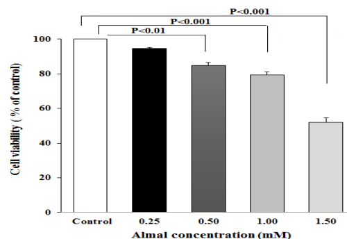
Figure 1. Effects of aluminium maltolate (Almal) on cell viability of PC12 cells using MTT assay. Treatment with different concentrations of Almal (0-1.5 mM) reduced viability of PC12 cells dose dependently. The represented data are mean±SD of at least three independent experiments and were analyzed using one way ANOVA followed by Tukey's post hoc test
