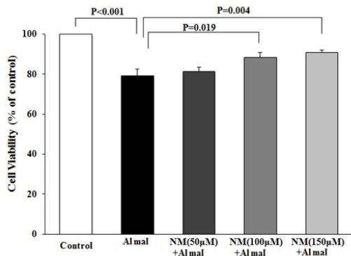
Figure 2. The effect of nimodipine (NM) on aluminum maltolate (Almal)-induced Cell death. PC12 cells were treated with Almal (1 mM) in the absence or presence of NM (50, 100, 150 µm). Cell viability was then evaluated using MTT assay. The represented data are mean±SD of at least three independent experiments and were analyzed using one way ANOVA followed by Tukey's post hoc test
